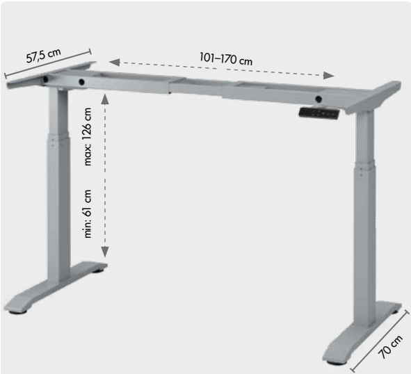
Frame with electric height-regulation NTX1000
