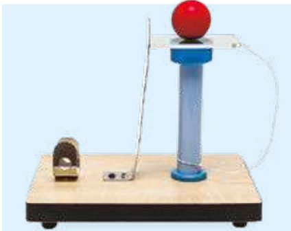
A device for demonstrating the inertia of bodies HG0106
