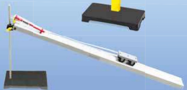
Uniform motion and uniformly accelerated motion. Demonstration set QH 0053
